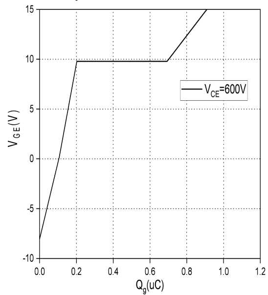
栅极电荷特性, IGBT, 逆变器 (典型) Gate charge characteristic, IGBT, Inverter (typical)
